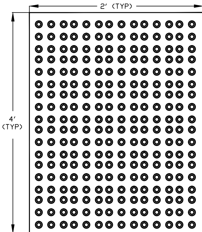
DETECTABLE WARNING TRUNCATED DOME
